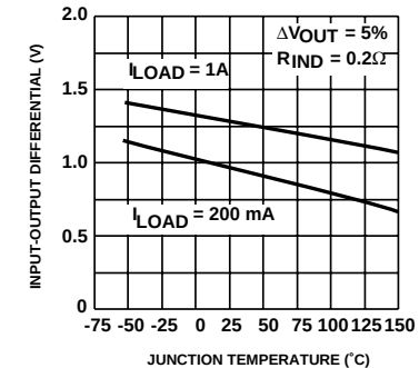
Dropout Voltage
