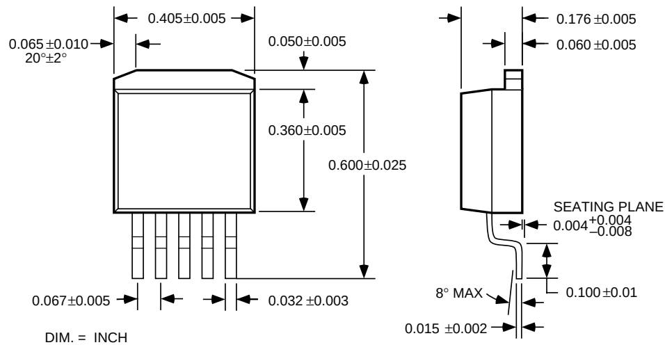
5-Lead TO-263 (T)
