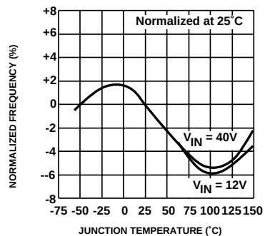
Oscillator Frequency
