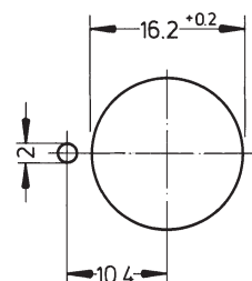
Panel cut-out
