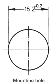
Mounting hole
