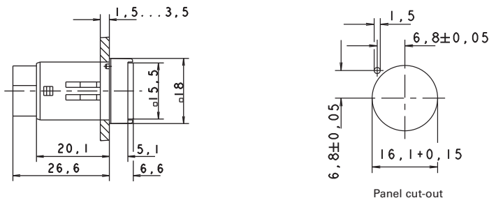
Panel cut-out
