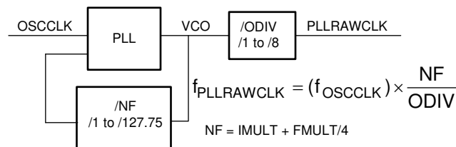
Figure 7-16. System PLL
