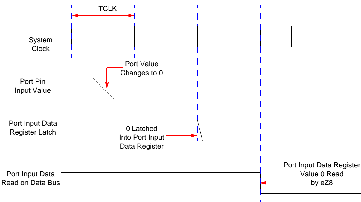
Figure 34. Port Input Sample Timing
