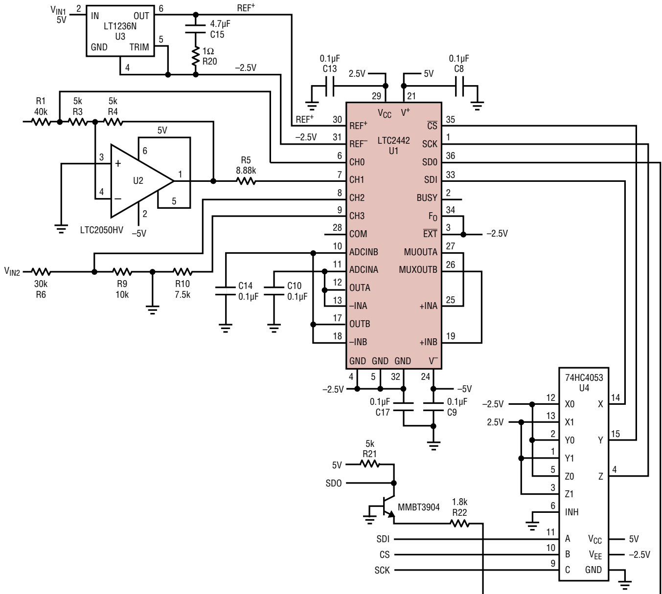
Figure 20. Scaling Inputs for \pm 10V Range
