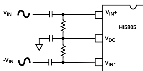
FIGURE 3. AC COUPLED DIFFERENTIAL INPUT
