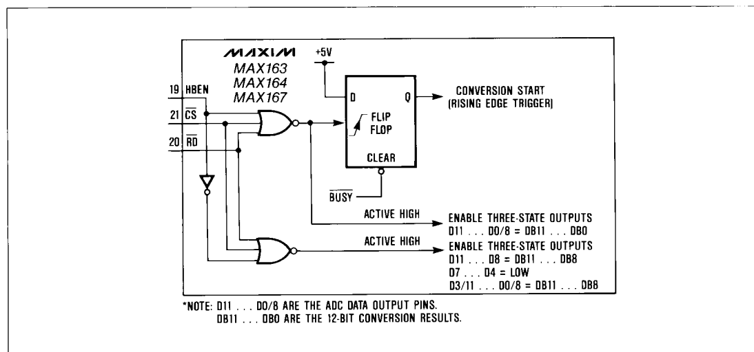
Figure 8. Logic Equivalent for \overline{RD} , \overline{CS} and \overline{HBEN} Inputs
