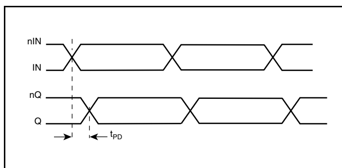
Propagation Delay
