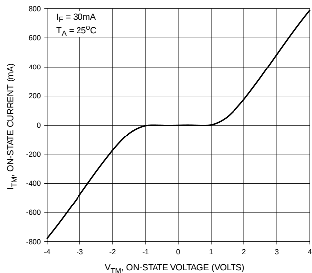
Figure 2. On-State Characteristics
