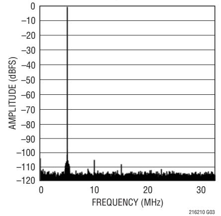
LTC2162: 64k Point FFT, f_{IN} = 5\text{MHz} , -1dBFS, 65Msps
