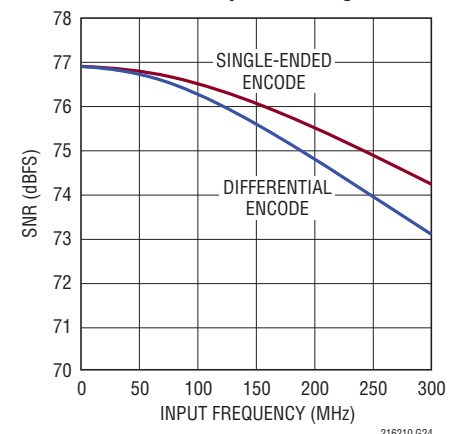
LTC2161: SNR vs Input Frequency, -1\text{dBFS} , 40\text{Mps} , 2\text{V} Range
