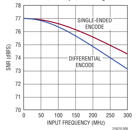
LTC2162: SNR vs Input Frequency, -1dBFS, 65Msps, 2V Range
