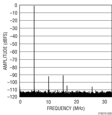
LTC2162: 64k Point FFT, f_{IN} = 70\text{MHz} , -1dBFS, 65Msps
