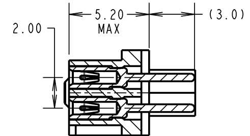
SECTION X-X
