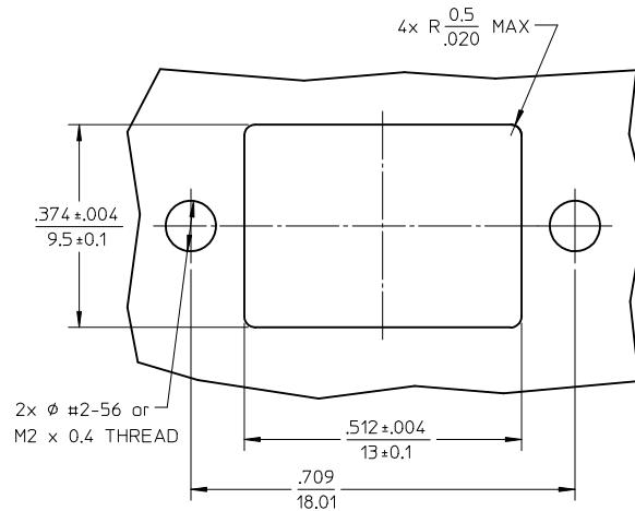
RECOMMENDED MOUNTING PATTERN
