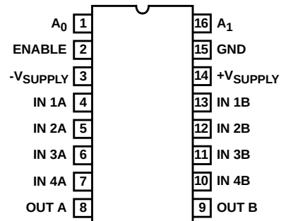
HI1-0549 (CERDIP), HI3-0549 (PDIP), HI9P0549 (SOIC)
