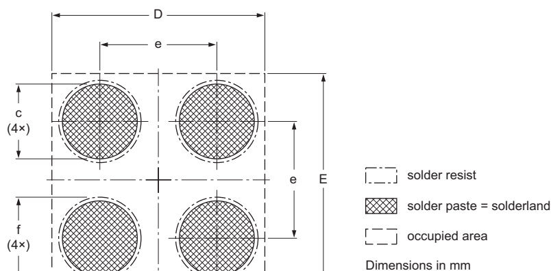
Fig 39. Soldering footprint WLCSP4
