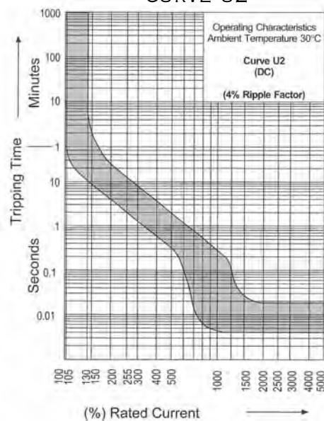
UL 489A RATED CURVE U2
