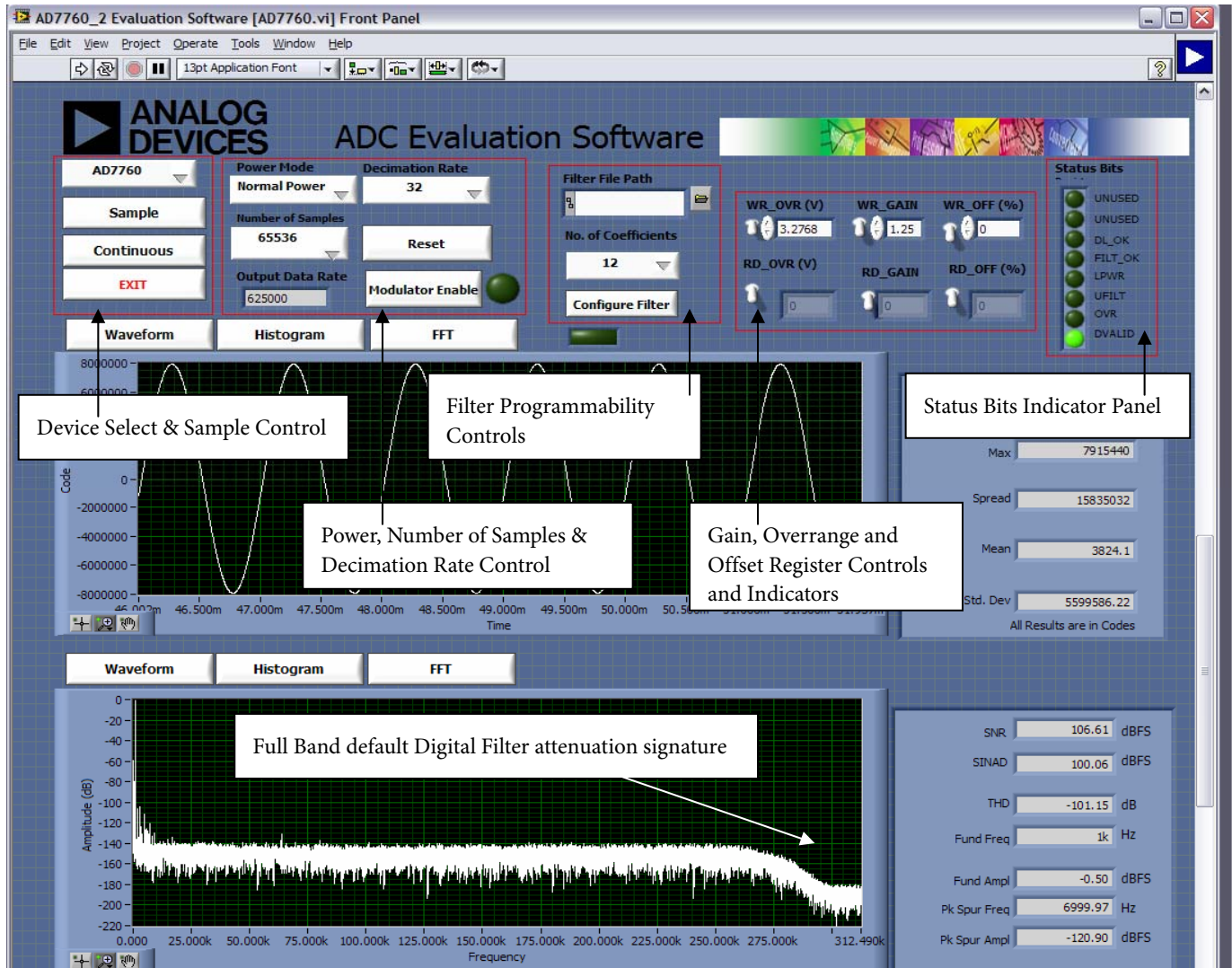
Figure 10. Front Panel GUI showing control and indicator information and the performance with a -0.5\text{dB} 1\text{kHz} input tone in decimate by 32 mode when running with the default 40\text{MHz} MCLK.
