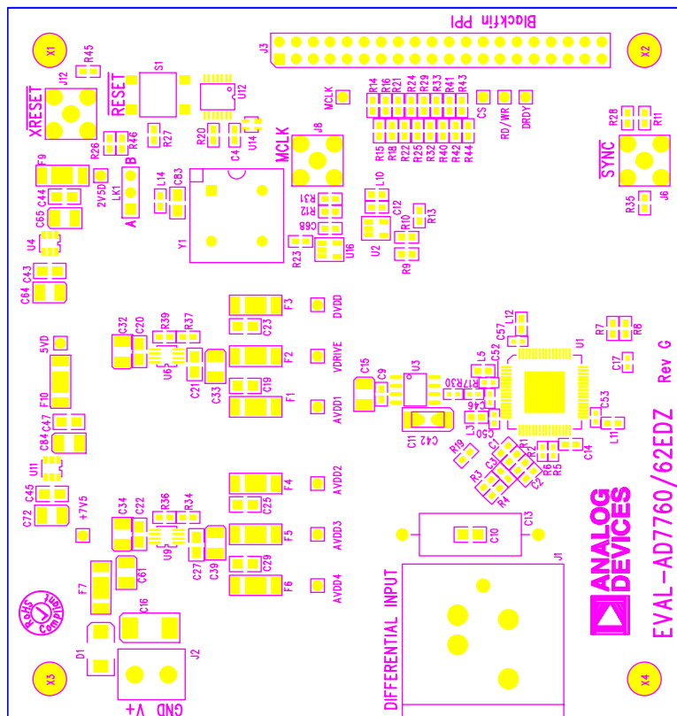
EVAL-AD7760/62EDZ (Rev. G) – Component Side View Silkscreen Top
