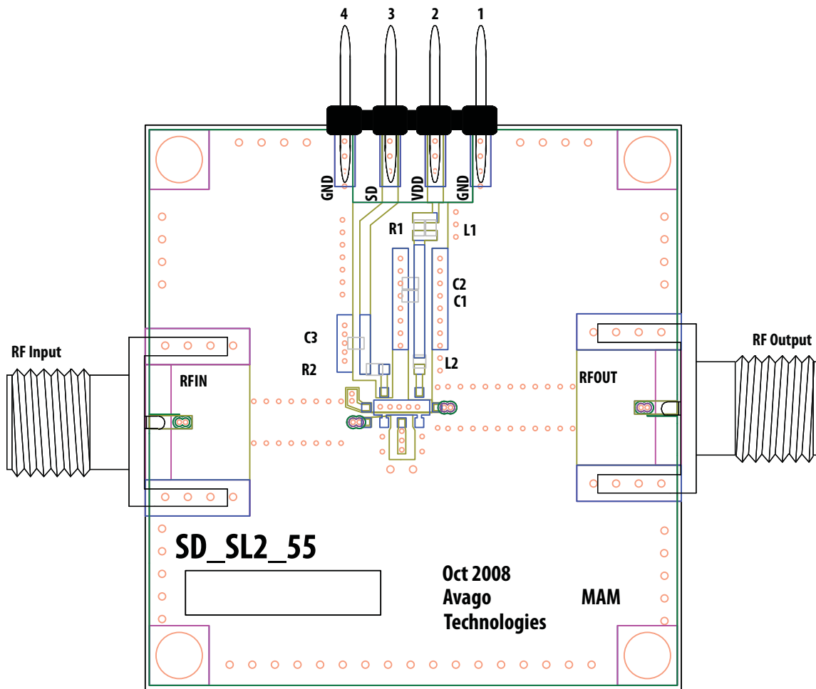
DC Pin Configuration of 4-pin connector
