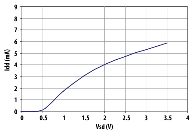
Figure 7. Idd vs Vsd for Vdd = 1.8V, R2 = 3.9k 0hm
