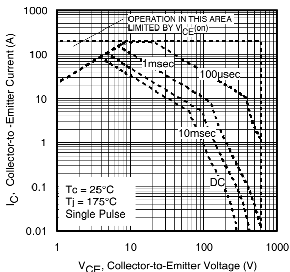
Fig. 4 - Forward SOA
