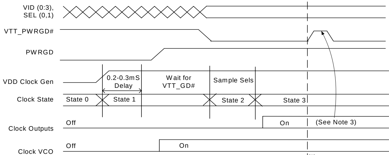
Figure 6. VTT_PWRGD# Timing Diagram (with P4 Mode, SELP4 K7 = 1 ) [3]
