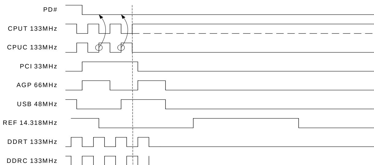
Figure 2. Power-down Assertion Timing Waveform (in P4 Mode)
