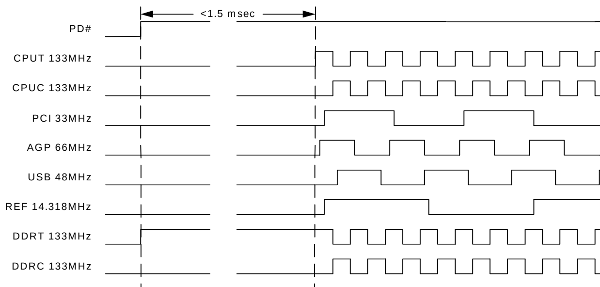
Figure 5. Power-down Deassertion Timing Waveform (in K7 Mode)
