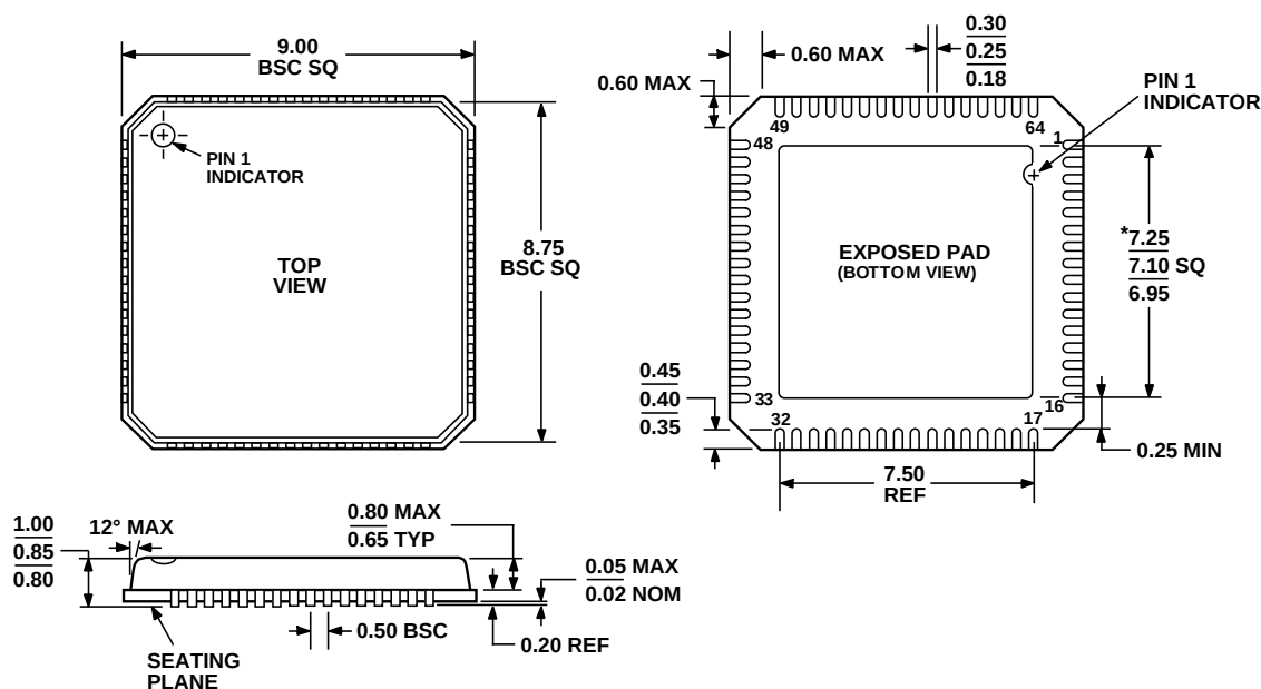
Figure 14. 64-Lead Free Chip Scale Package [LFCSF] (CP-64-3)
