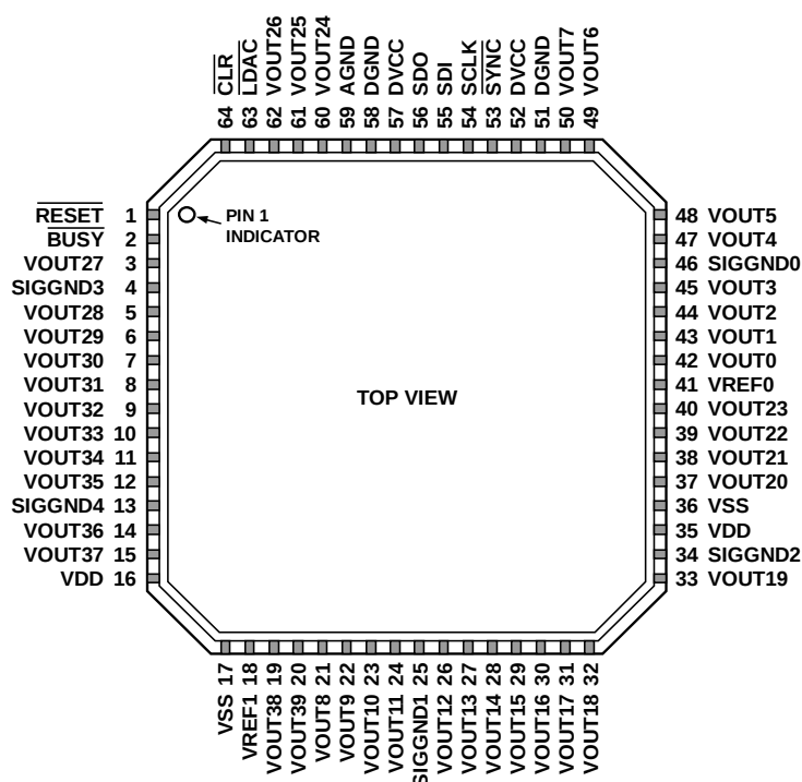
Figure 7.64-Lead LFCSP Pin Configuration
