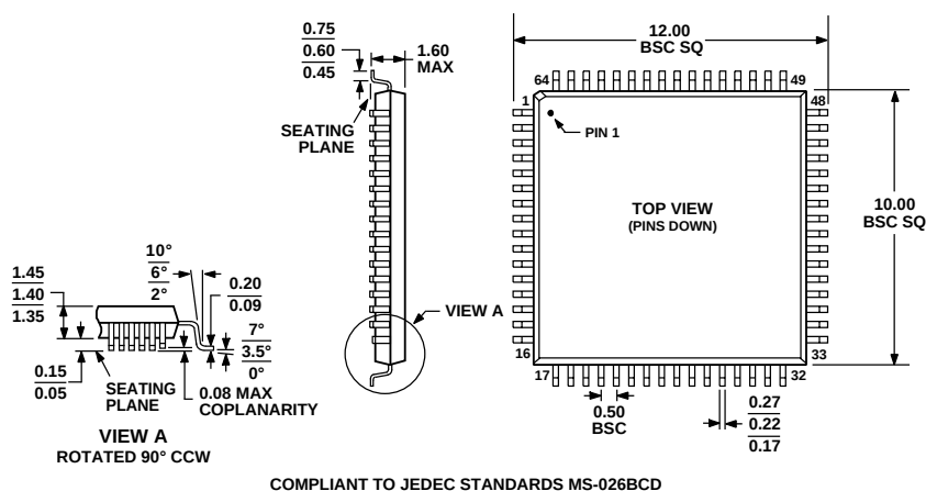
Figure 13. 64-Lead Low Profile Quad Flat Package [LQFP] (ST-64-2)
