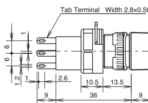
Solder/Tab Terminal
