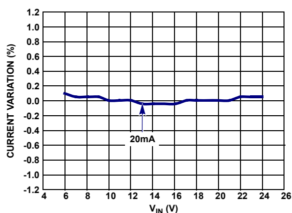
FIGURE 6. CURRENT REGULATION
