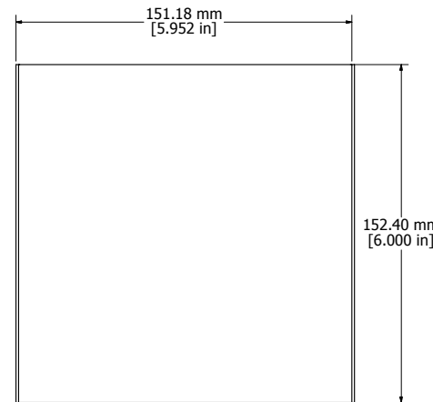
BOTTOM/TOP ENCLOSURE
