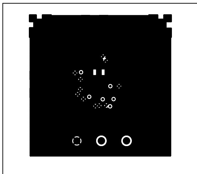
Figure 6. MAX2039 EV Kit PC Board Layout—Inner Layer 2 (GND)
