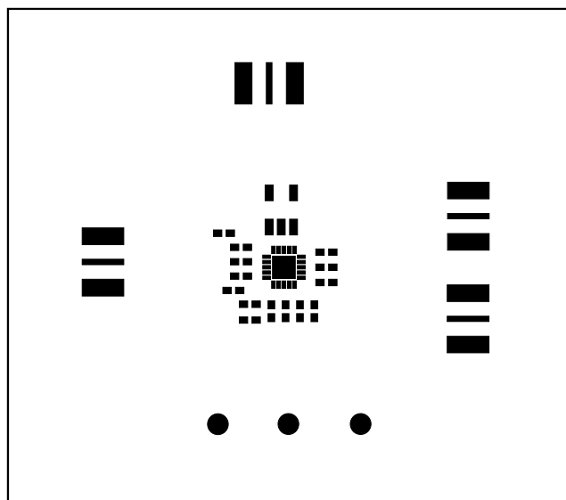
Figure 4. MAX2039 EV Kit PC Board Layout—Top Soldermask
