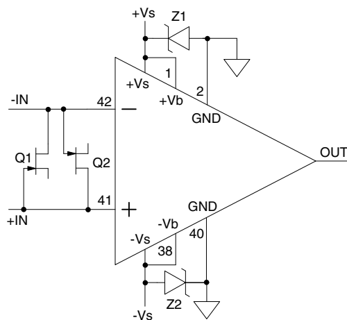
FIGURE 1: OVERVOLTAGE PROTECTION
