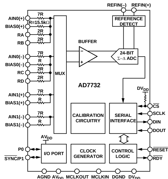
Figure 12. Block Diagram
