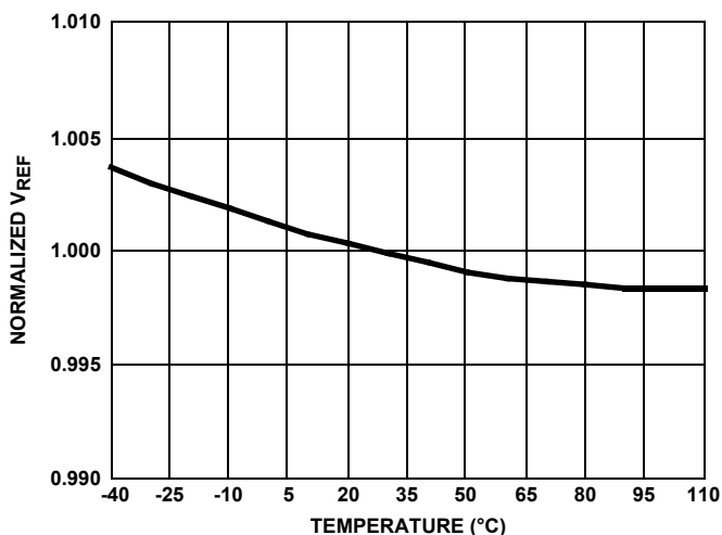
FIGURE 6. VREF vs TEMPERATURE
