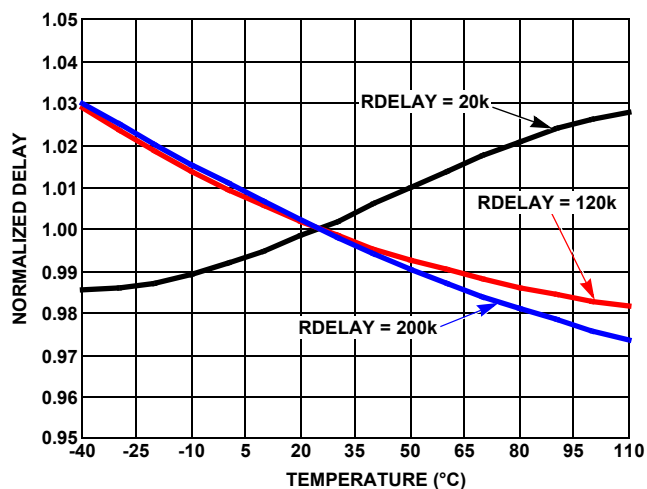
FIGURE 4. DELAY TIME vs TEMPERATURE (OVERLAP)
