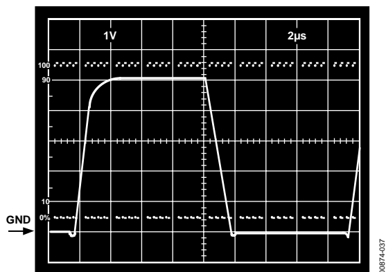
Figure 37. V_S = 5\text{ V} , 0\text{ V} ; Unity Gain Follower Response to 0\text{ V} to 5\text{ V} Step
