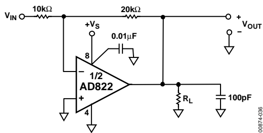
Figure 36. Gain-of-T2 Inverter
