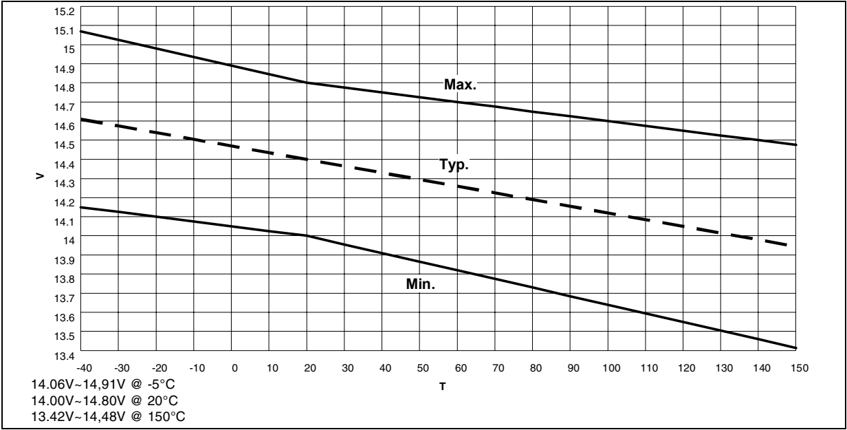
Figure 4. Vreg-2
