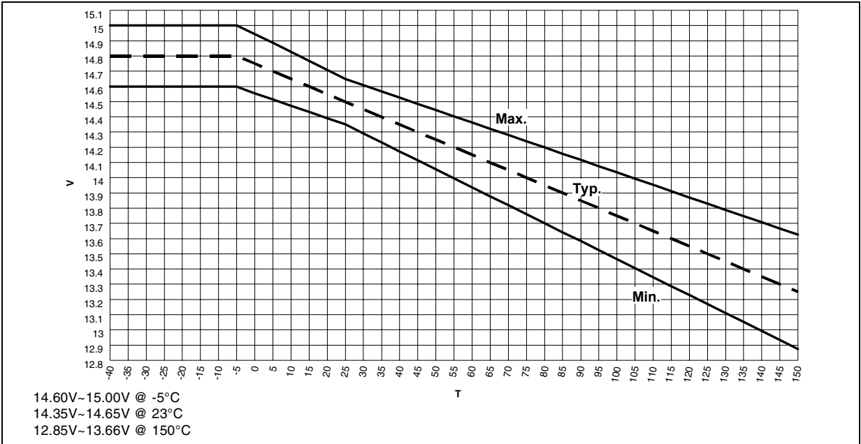
Figure 4. Vreg-2
