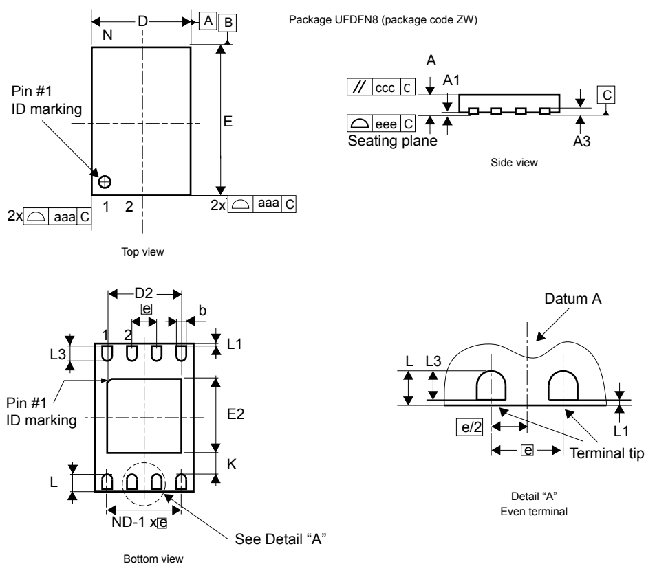
Figure 15. UFDFPN8 - Outline
