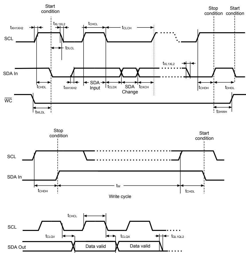
Figure 12. AC waveforms
