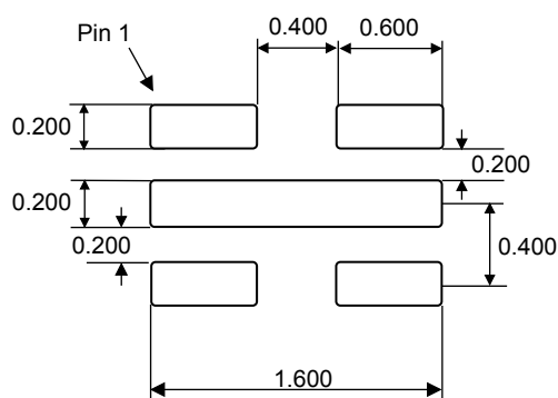
Figure 14. UDFPN5 - Recommended footprint
