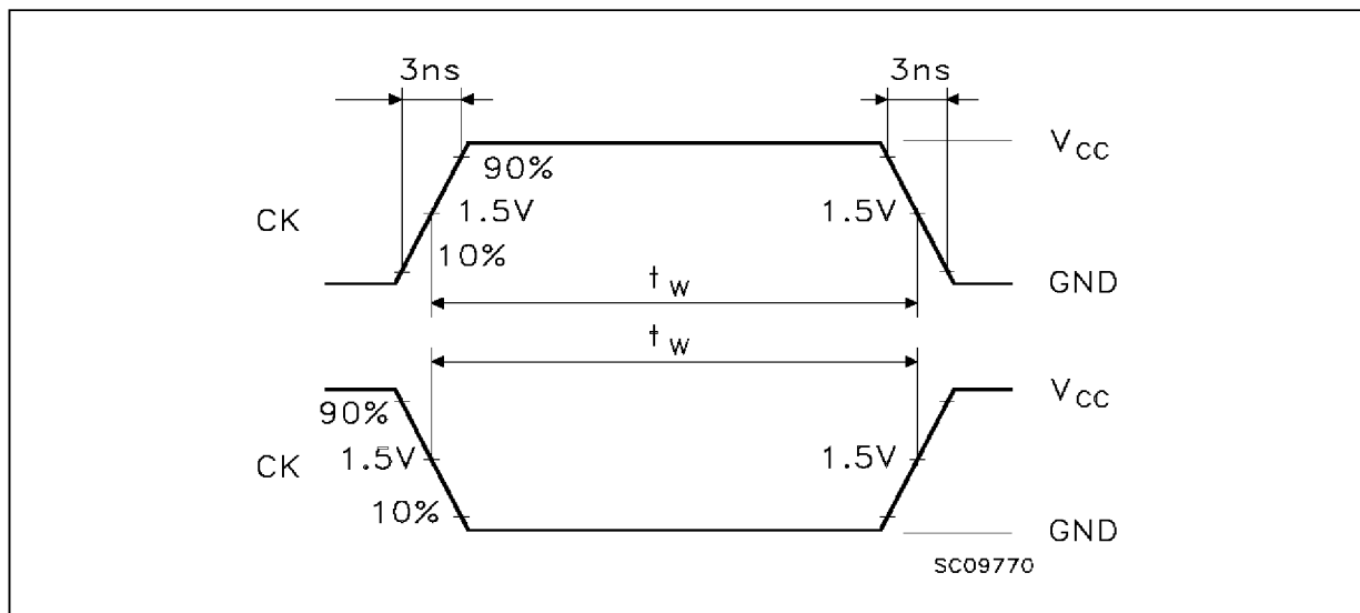
WAVEFORM 3: PULSE WIDTH
