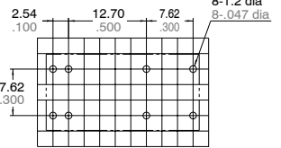
PC board pattern (Bottom view) Single side stable 1 coil latching type
