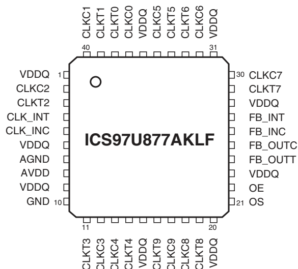
40-Pin MLF
