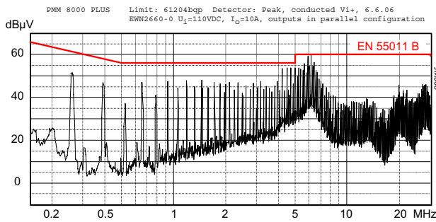
Fig. 13a Conducted emissions of EW models: Disturbances (peak) at the phase input according to EN 55011, measured at V_{i \text{ nom}} and I_{o \text{ nom}} . (EWN2660-0)
