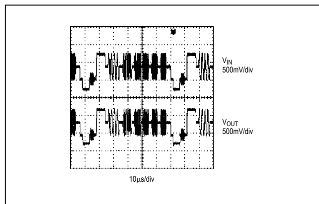
Figure 3. Multiburst Response
