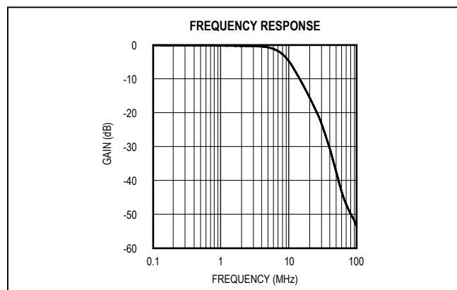
Figure 2. Frequency Response
