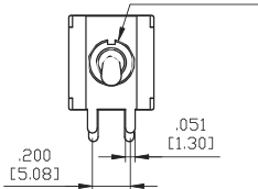
M7 Double Pole .244 DIA [6.20]
