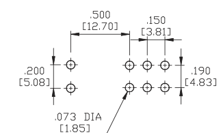
P.C.MOUNTING
