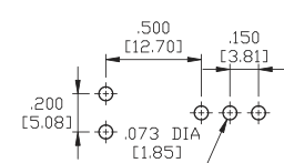
P.C.MOUNTING
