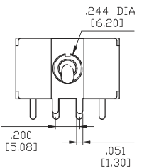
M7 Four Pole .244 DIA [6.20]
