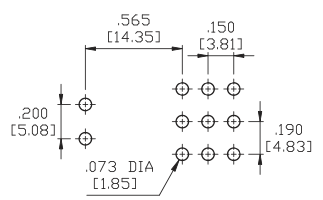
P.C.MOUNTING
