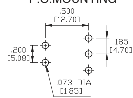
P.C.MOUNTING
