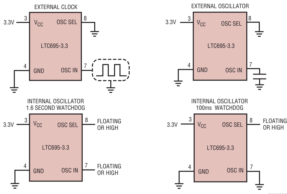
Figure 12. Oscillator Configurations
