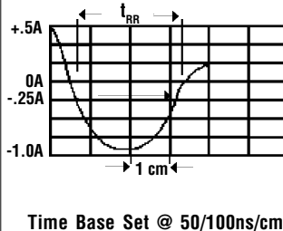
Reverse Recovery Characteristics
