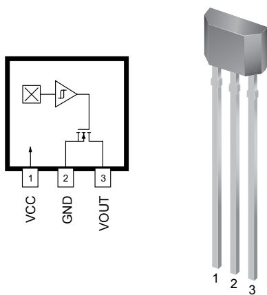
Package UA, 3-pin SIP
