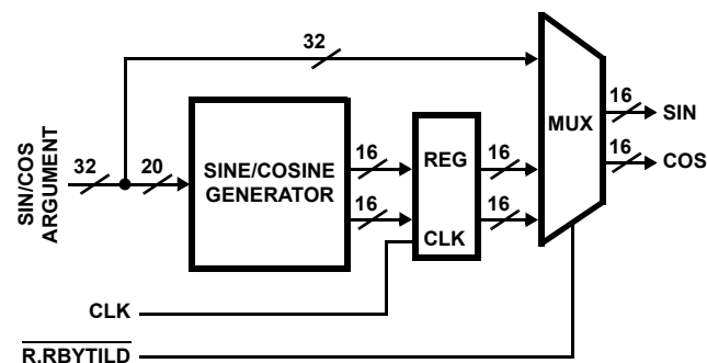
FIGURE 2. SINE/COSINE SECTION
