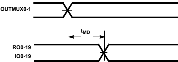
FIGURE 10. MULTIPLEXER TIMING
