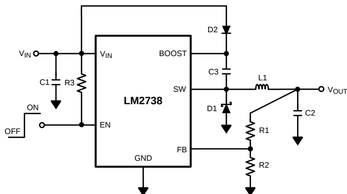
Figure 39. LM2738Y (550 kHz) V_{\text{BOOST}} Derived from V_{\text{IN}} 5 V to 1.5 V / 1.5 A
