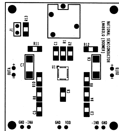
FIGURE 7. Recommended LQ PC board layout: Component-side Silkscreen
