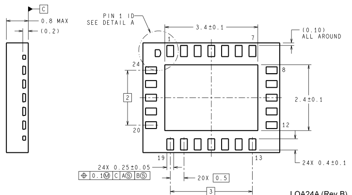
24-Lead Molded pkg, Leadframe Package LLP Order Number LM4863LQ NS Package Number LQA24A
