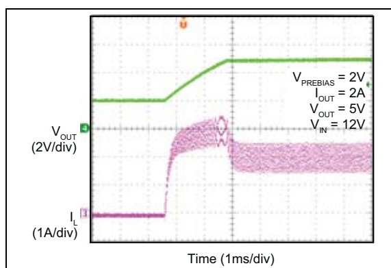
FIGURE 2-48: V_{IN} Start-up w Pre-Biased Output (MIC28512-1).
