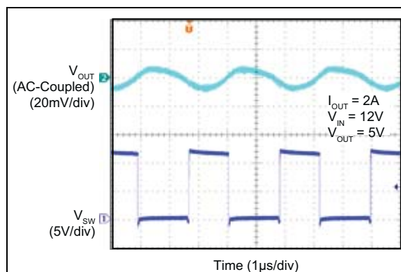
FIGURE 2-52: MIC58512-2 Switching Waveform.
