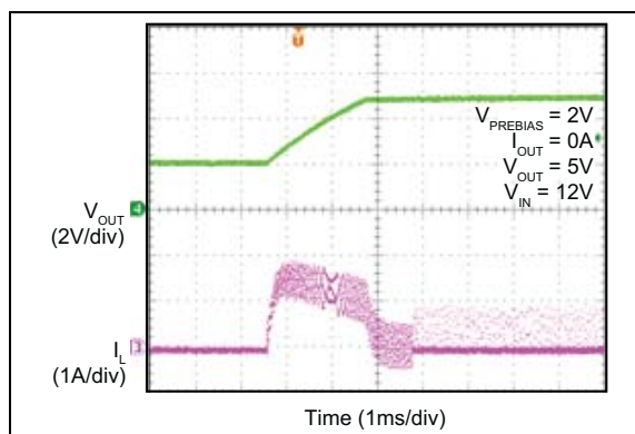
FIGURE 2-47: V_{IN} Start-up w Pre-Biased Output (MIC28512-1).
