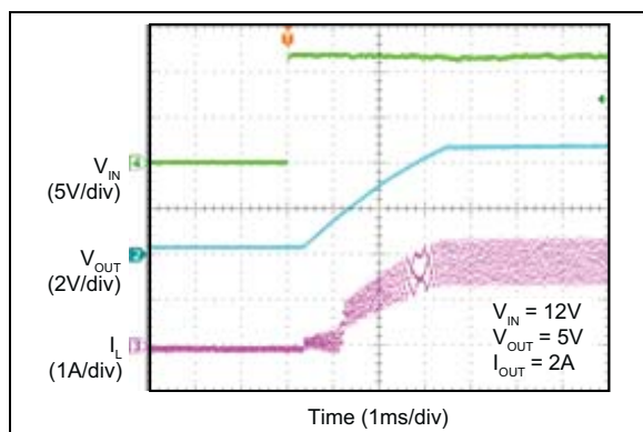
FIGURE 2-43: V_{IN} Soft Start Turn-On (MIC28512-1).
