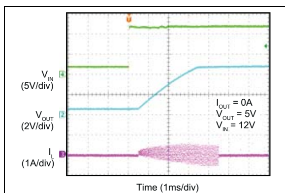
FIGURE 2-45: Soft Start (MIC28512-1).
