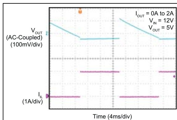
FIGURE 2-53: MIC28512-1 Transient Response.
