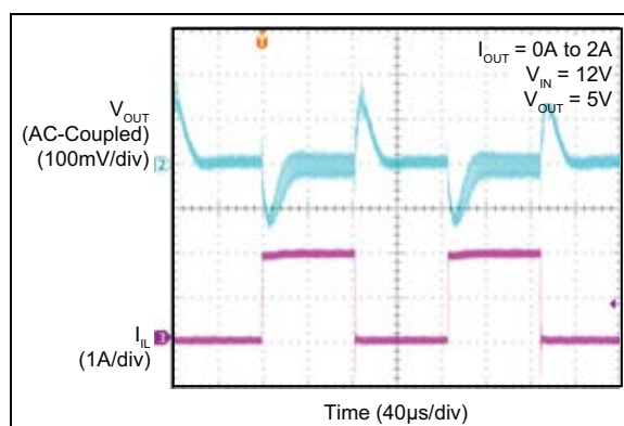
FIGURE 2-54: MIC28512-2 Transient Response.
