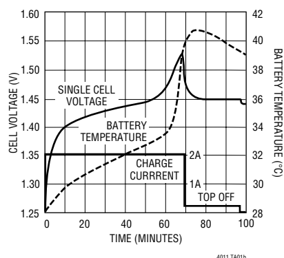
Typical NiMH Charge Cycle at 1C
