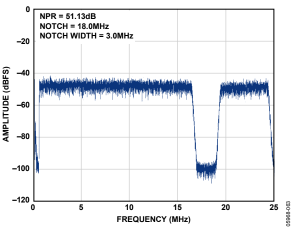
Figure 40. Noise Power Ratio (NPR), AD9212-65
