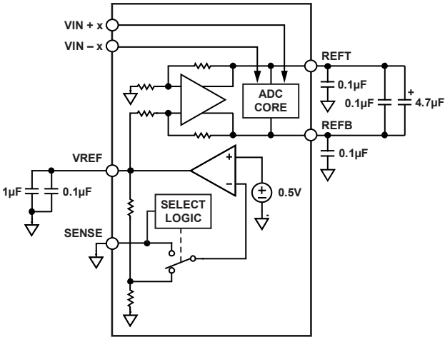
Figure 63. Internal Reference Configuration
