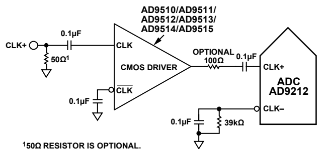
Figure 54. Single-Ended 1.8 V CMOS Sample Clock
