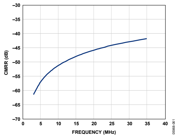
Figure 38. CMRR vs. Frequency, AD9212-65
