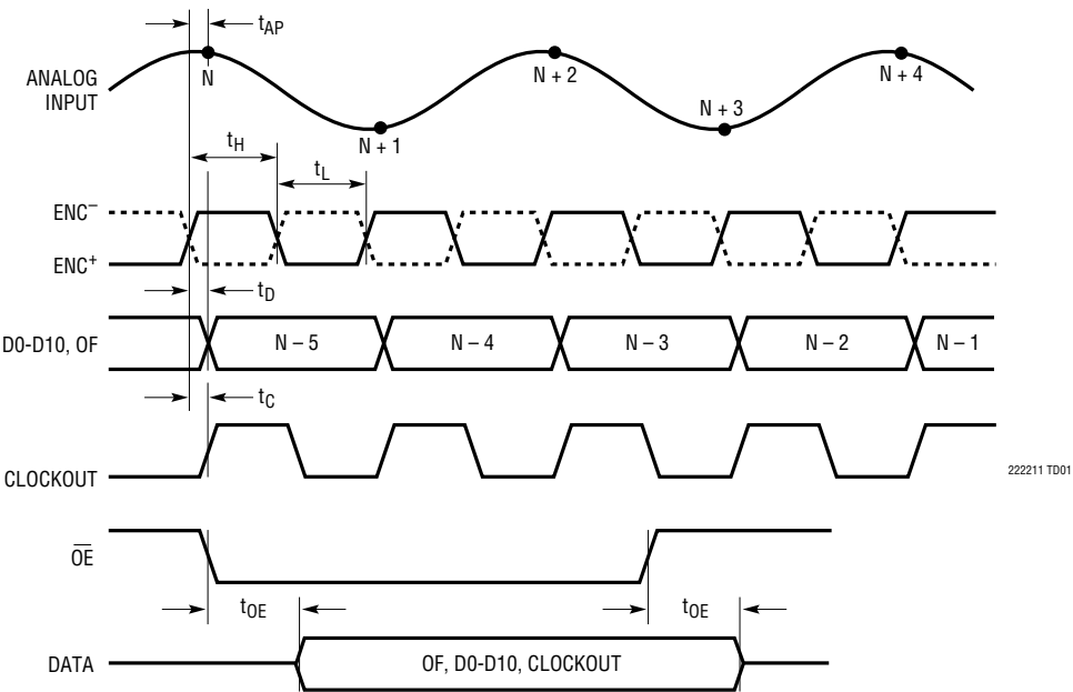
Timing Diagram
