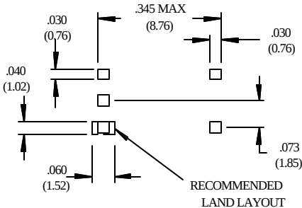
PWB FOOTPRINT
