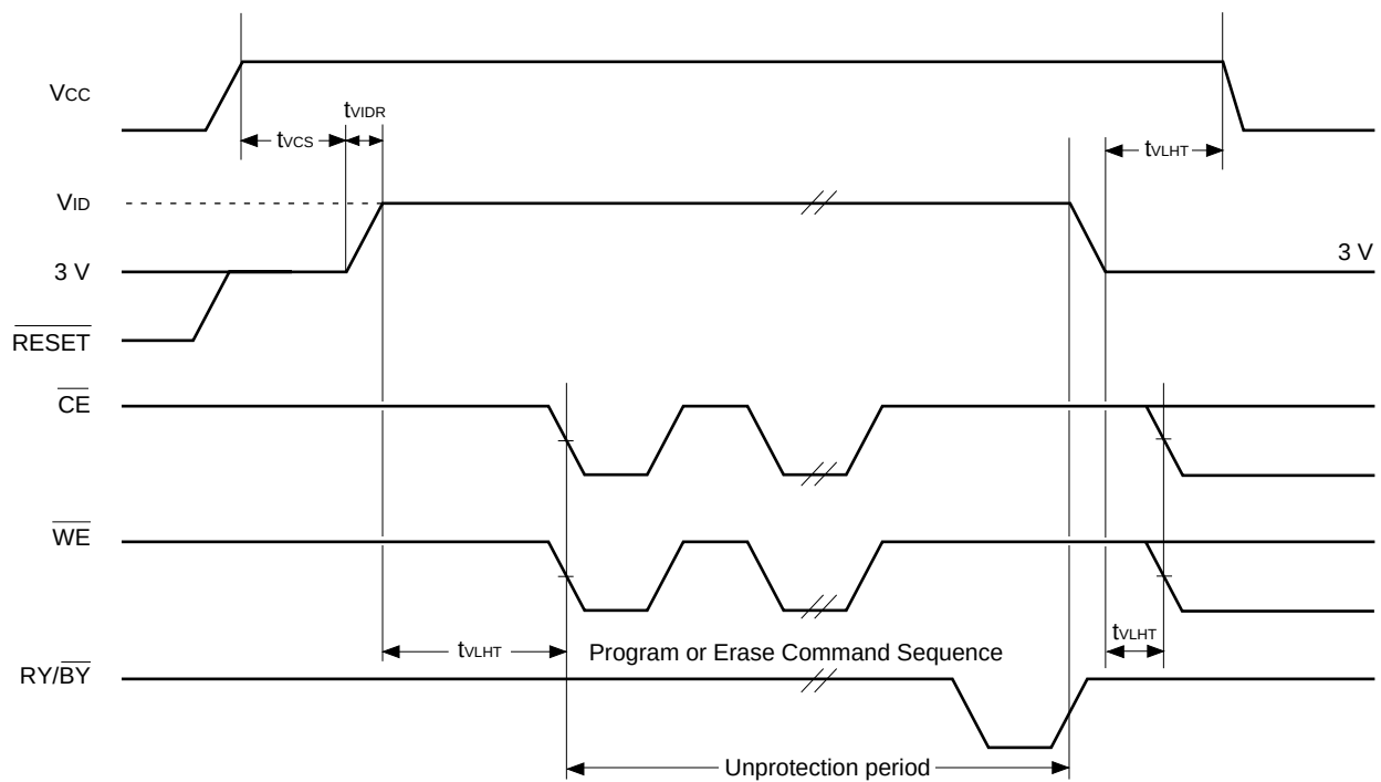
Figure 14 Temporary Sector Unprotection Timing Diagram
