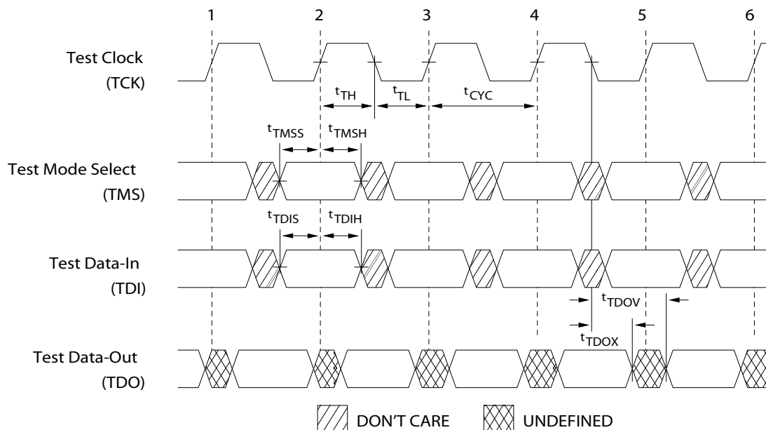
Figure 3. TAP Timing
