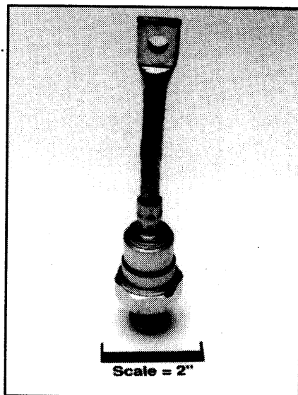
R602__22/R603__22 Fast Recovery Rectifier 220 Amperes Average, 1600 Volts
